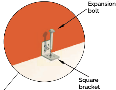
Anchoring detail.
